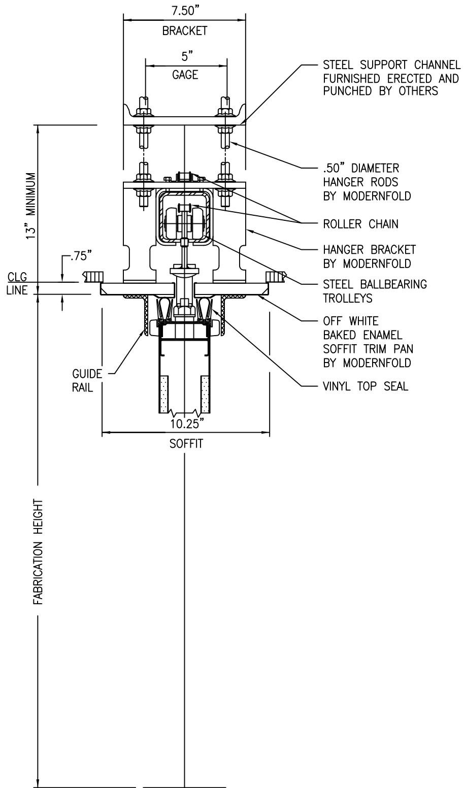
#14 TRACK / ELECTRIC / STEEL CHANNEL
