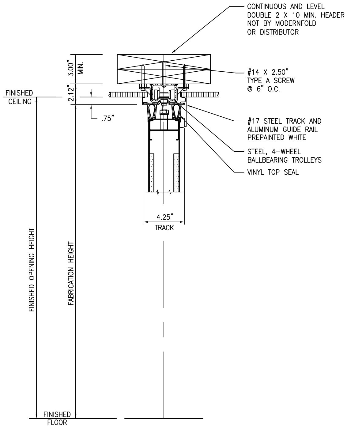
#17 TRACK / DIRECT MOUNT / GUIDERAIL
