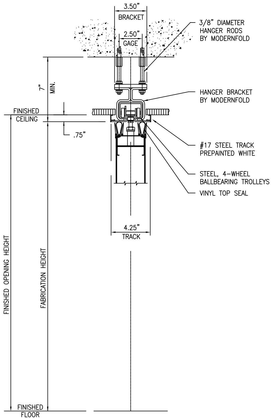
#17 TRACK / HEAVY DUTY (2.5 GUAGE) BRACKETS / CONCRETE ANCHORS
