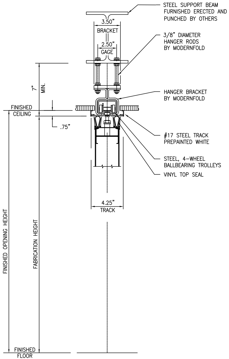
#17 TRACK / HEAVY DUTY (2.5 GUAGE) BRACKETS / STEEL BEAM
