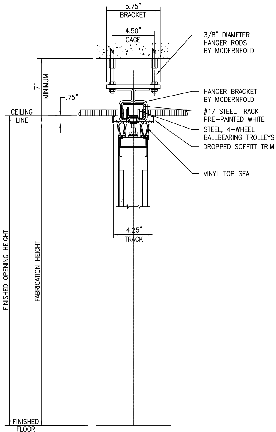
#17 TRACK / HEAVY DUTY (4.5 GUAGE) BRACKETS / CONCRETE ANCHORS
