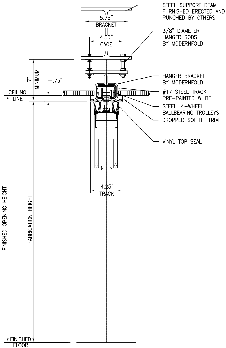
#17 TRACK / HEAVY DUTY (4.5 GUAGE) BRACKETS / STEEL BEAM
