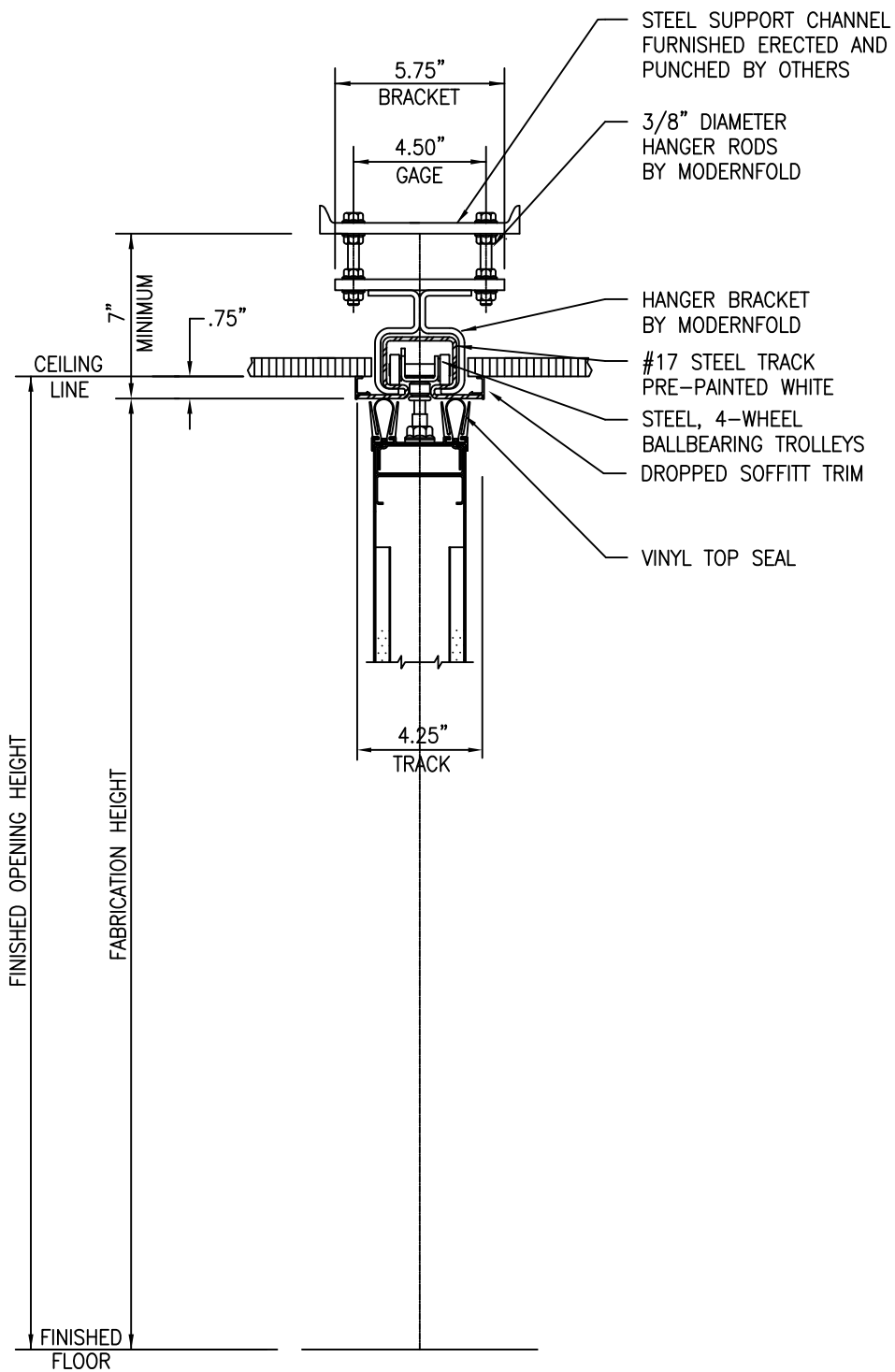
#17 TRACK / HEAVY DUTY (4.5 GUAGE) BRACKETS / STEEL CHANNEL
