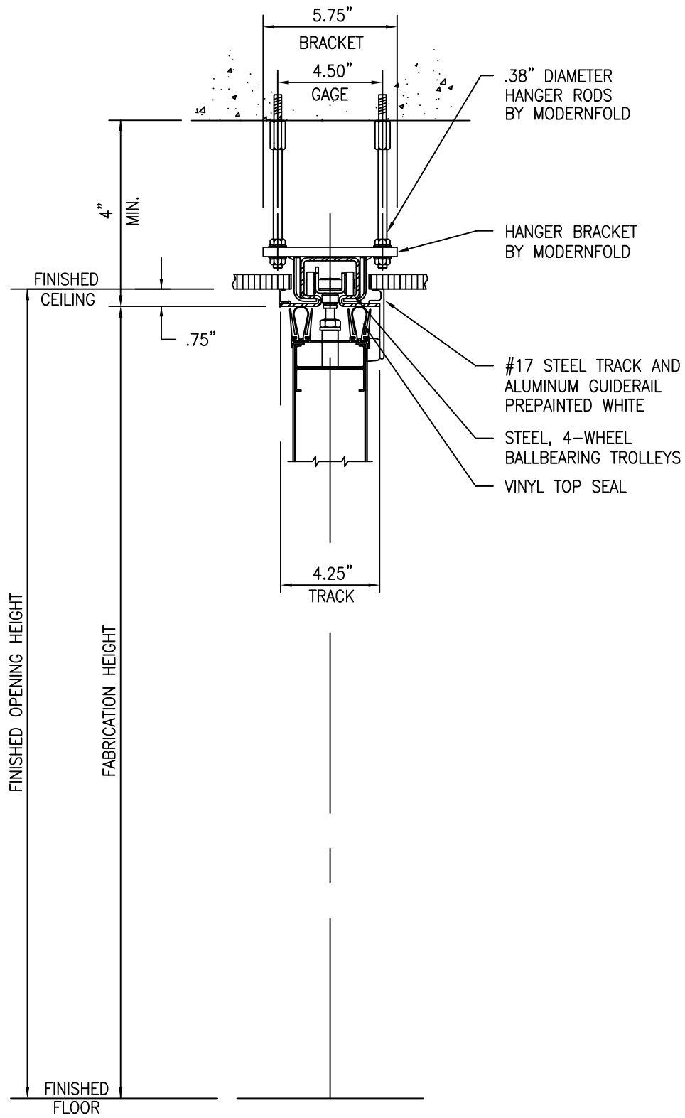
#17 TRACK / STANDARD BRACKETS / GUIDERAIL / CONCRET ANCHORS
