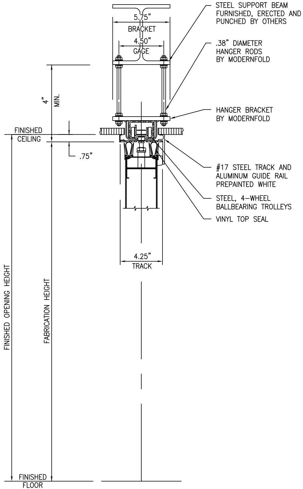
#17 TRACK / STANDARD BRACKETS / GUIDERAIL / STEEL BEAM
