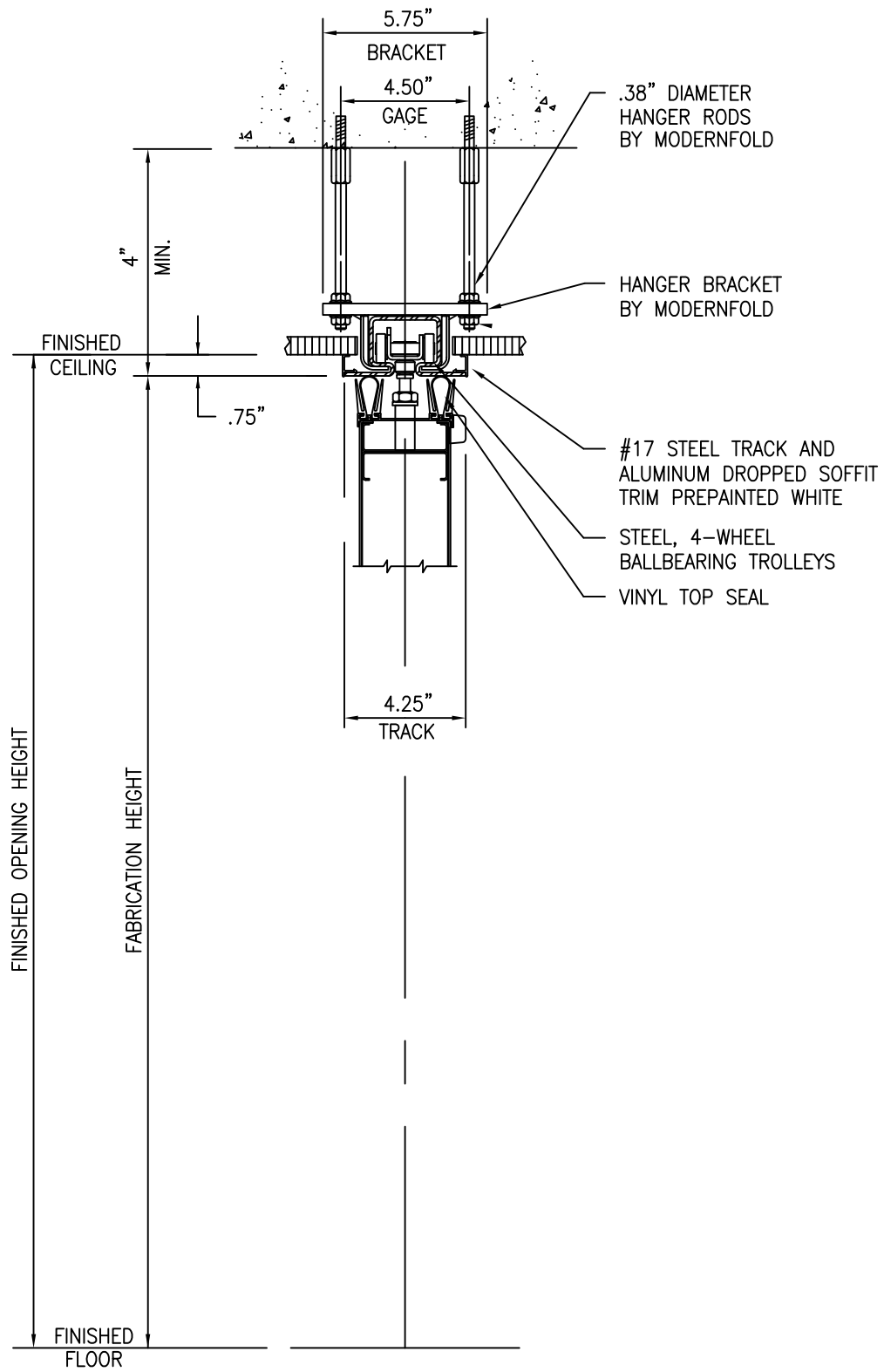
#17 TRACK / STANDARD BRACKETS / NO GUIDERAIL / CONCRETE ANCHORS
