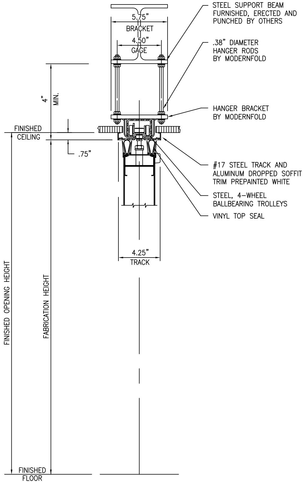
#17 TRACK / STANDARD BRACKETS / NO GUIDERAIL / STEEL BEAM
